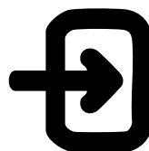
SAST/DAST
