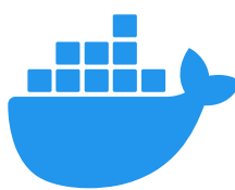
Docker
